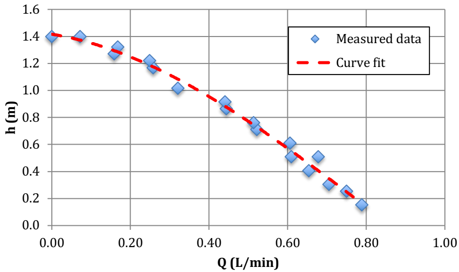
Figure 1 Measured head versus flow rate data from the pump experiment.
