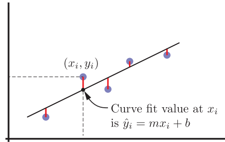
Figure 2: Geometry of a least squares line fit.
